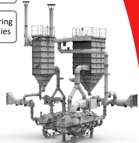
2 Vibrating Fluidized Beds Dryer-Cooler
